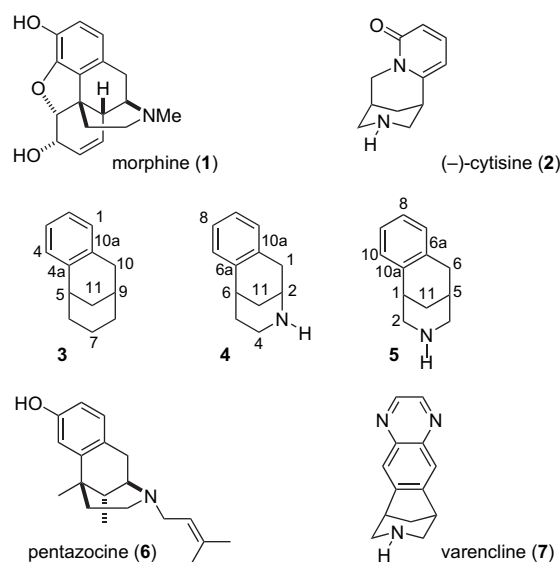
Figure 1. Structure of morphine ( 1 ) and cytisine ( 2 ), their common core 3 , the nitrogen-containing core structures 4 and 5 , as well as derived pharmaceuticals.
