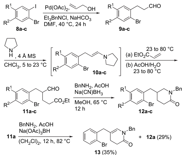
Scheme 1. Synthesis of the cyclization substrates 12a–c via reductive amination of the formyl esters 11a–c .
