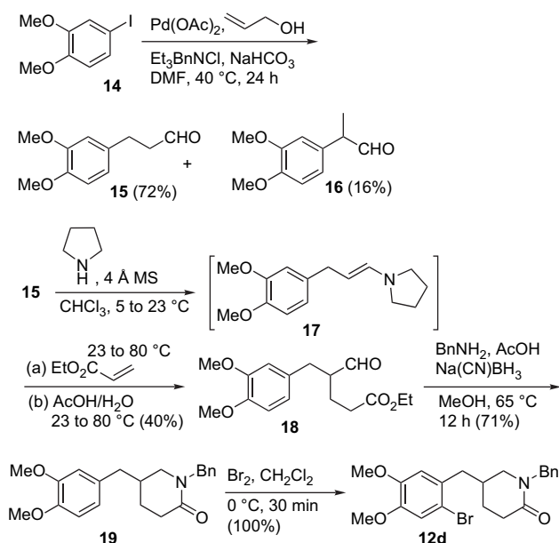
Scheme 2. Synthesis of piperidinone 12d from iodobenzene 14 .
