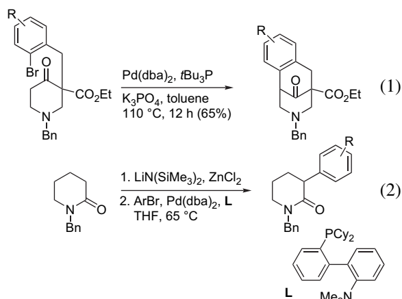
Figure 2. Intramolecular Buchwald–Hartwig arylation of ketones yielding 3-benzazocines (Eq. 1) and intermolecular lactam arylation (Eq. 2).
